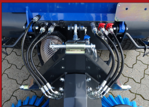
The sweeping front is built with a standard A-frame, and can be delivered with 2, 3 or 4 brushes.
