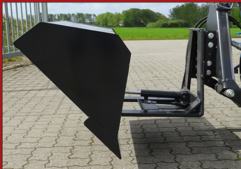
The front shovel is easy to empty, thanks to the strong, center mounted, hydraulic cylinder.
