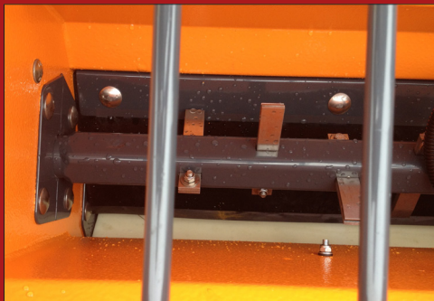
The spreader is equipped with a stainless stirring system, which ensures even distribution of the spreading material.
